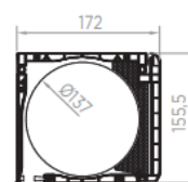
■ SC CURVE 185
