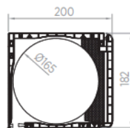
■ SC CURVE 200
